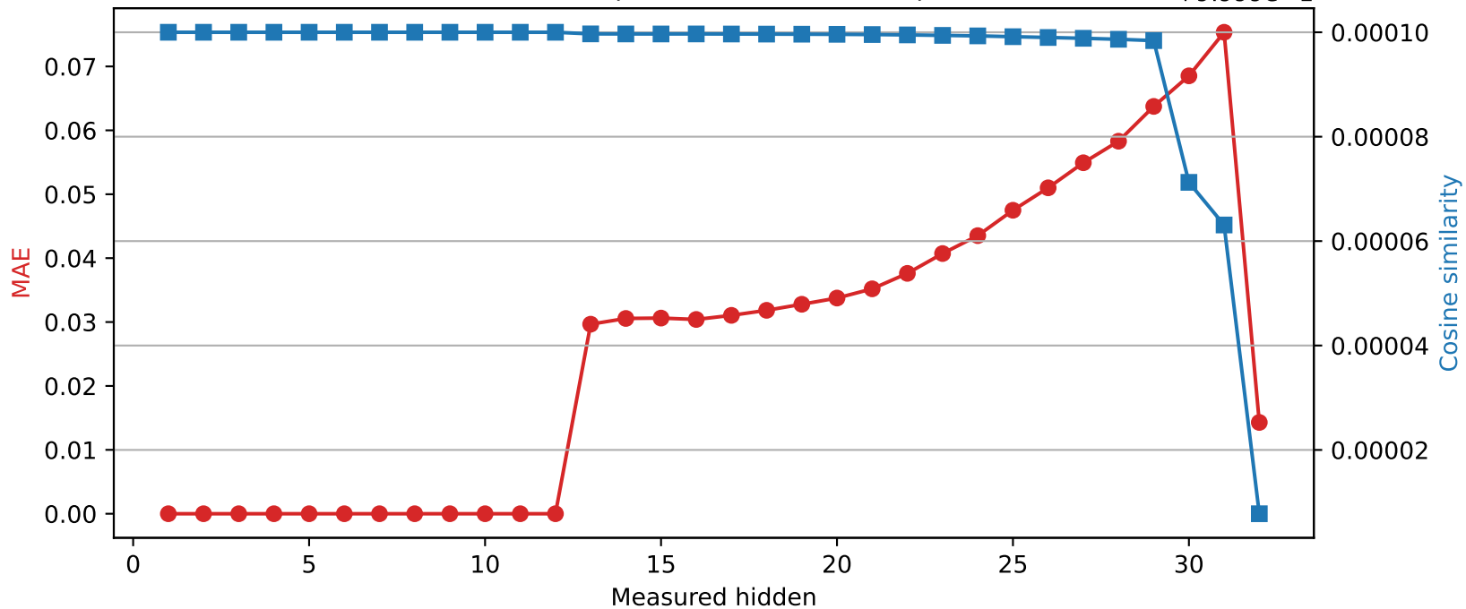
Phi-3-mini-4k-instruct | Quantized layer 12 | float16 \rightarrow int8
