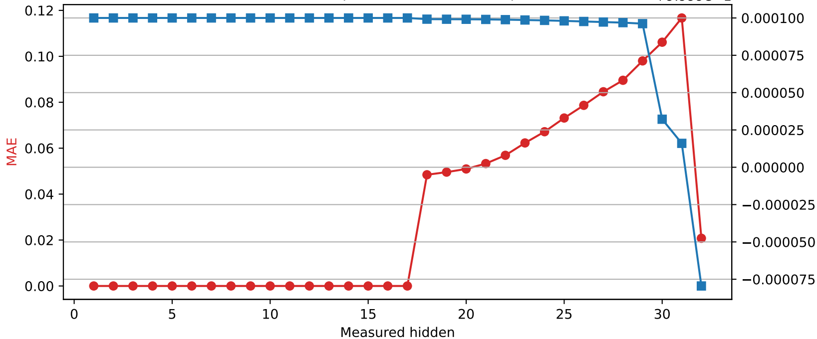
Phi-3-mini-4k-instruct | Quantized layer 17 | float16 \rightarrow int8
