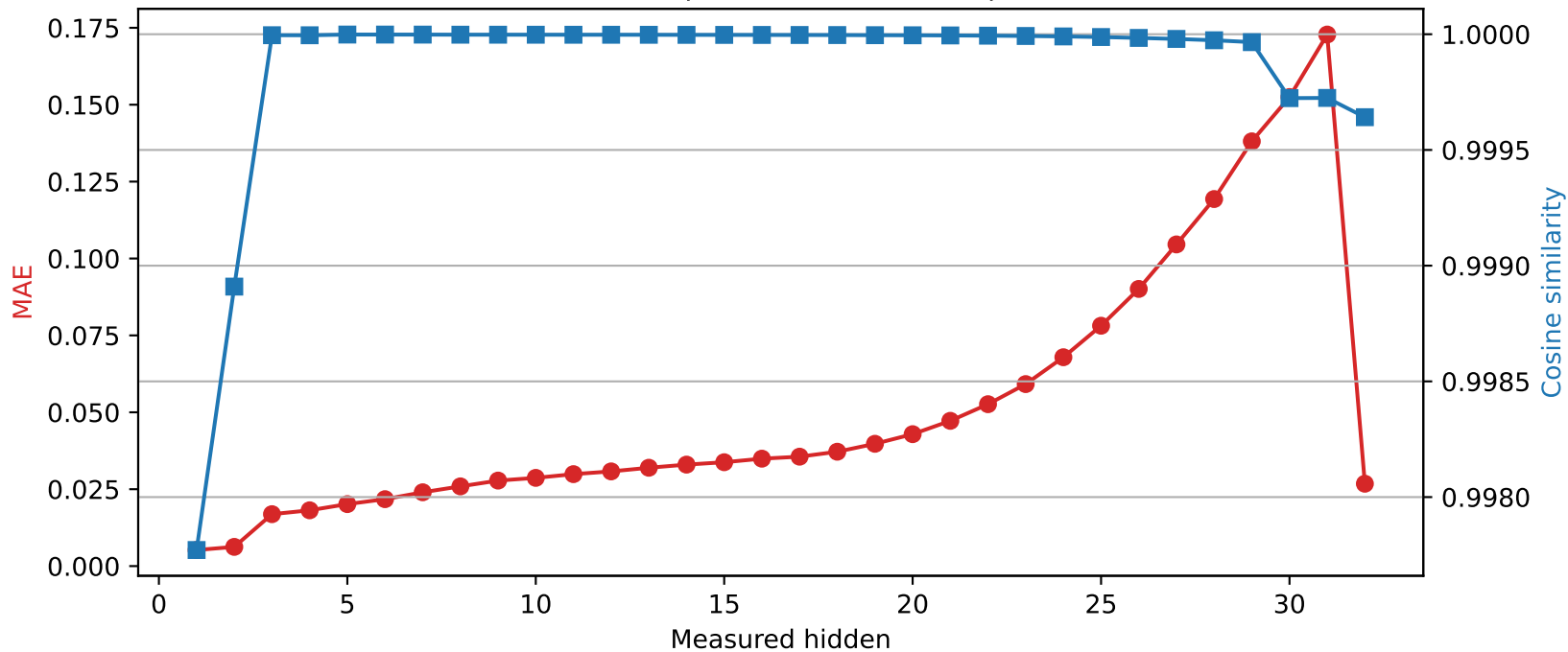
Phi-3-mini-4k-instruct | Quantized layer 0 | float16 \rightarrow int8
