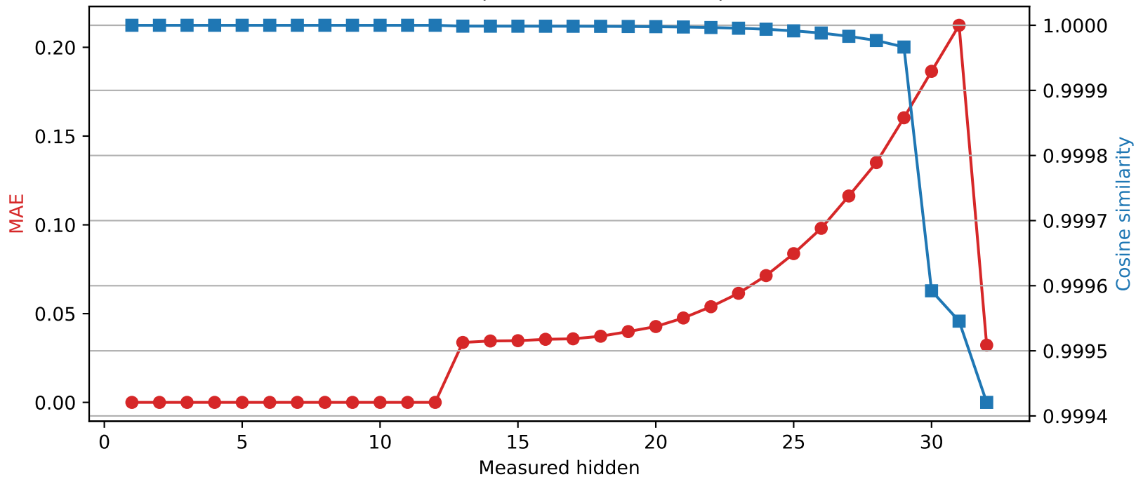
Phi-3-mini-4k-instruct | Quantized layer 12 | float16 \rightarrow int8
