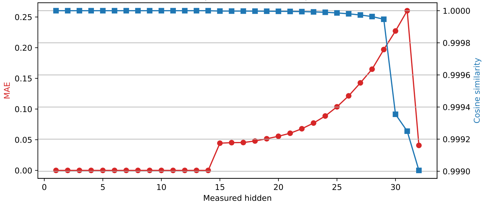
Phi-3-mini-4k-instruct | Quantized layer 14 | float16 \rightarrow int8
