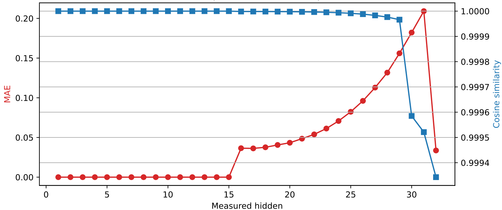
Phi-3-mini-4k-instruct | Quantized layer 15 | float16 \rightarrow int8
