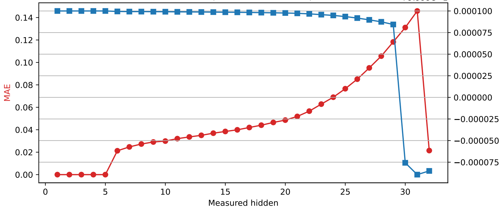
Phi-3-mini-4k-instruct | Quantized layer 5 | float16 \rightarrow int8
