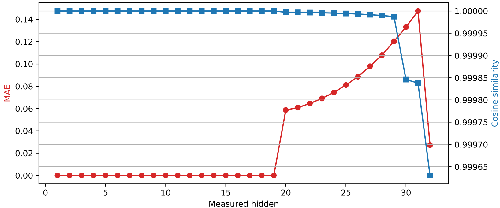
Phi-3-mini-4k-instruct | Quantized layer 19 | float16 → int8
