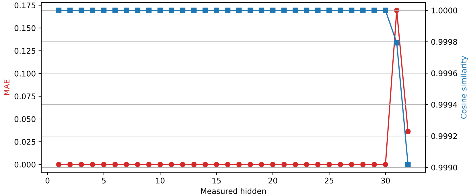
Phi-3-mini-4k-instruct | Quantized layer 30 | float16 \rightarrow int8
