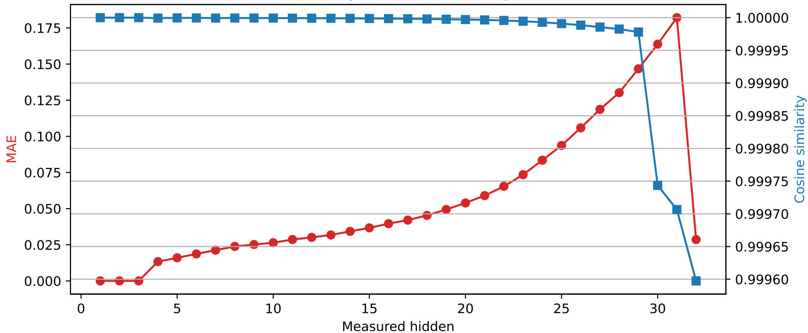
Phi-3-mini-4k-instruct | Quantized layer 3 | float16 → int8
