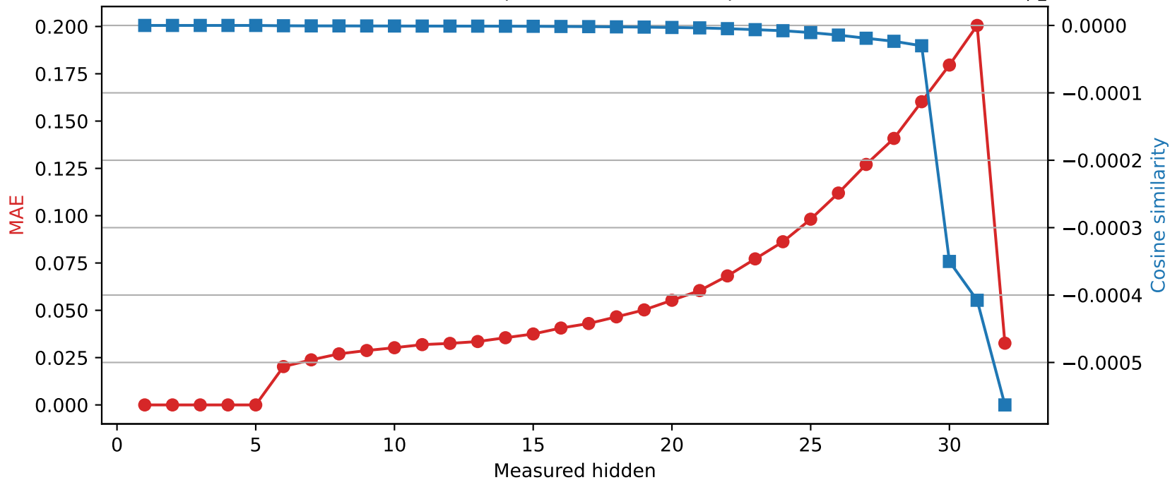
Phi-3-mini-4k-instruct | Quantized layer 5 | float16 → int8
