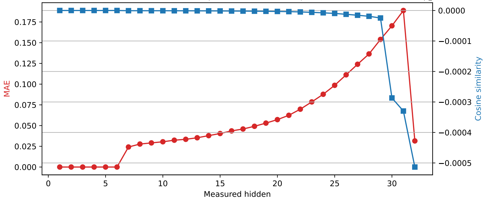
Phi-3-mini-4k-instruct | Quantized layer 6 | float16 → int8
