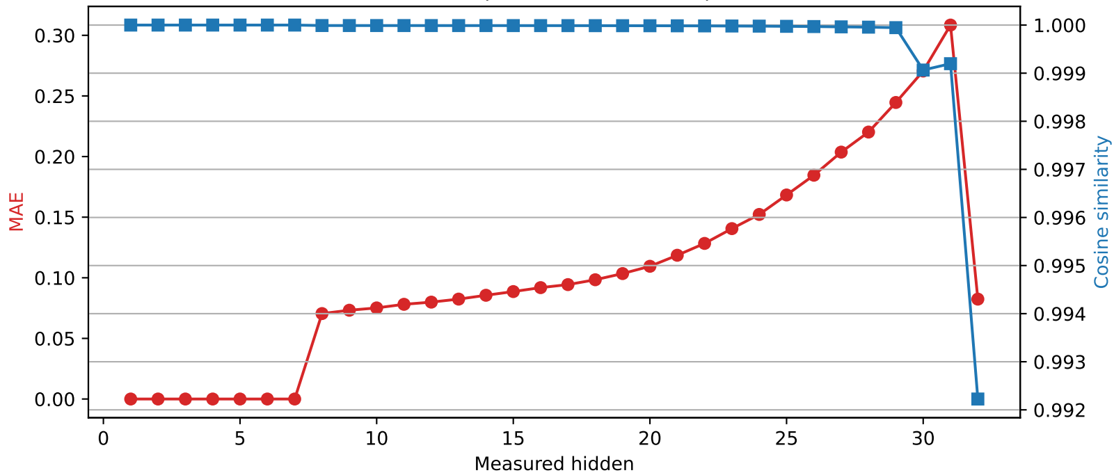
Phi-3-mini-4k-instruct | Quantized layer 7 | float16 \rightarrow int8
