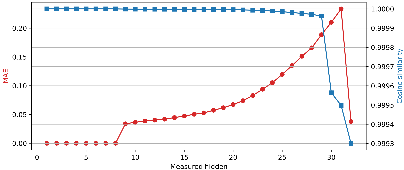
Phi-3-mini-4k-instruct | Quantized layer 8 | float16 \rightarrow int8
