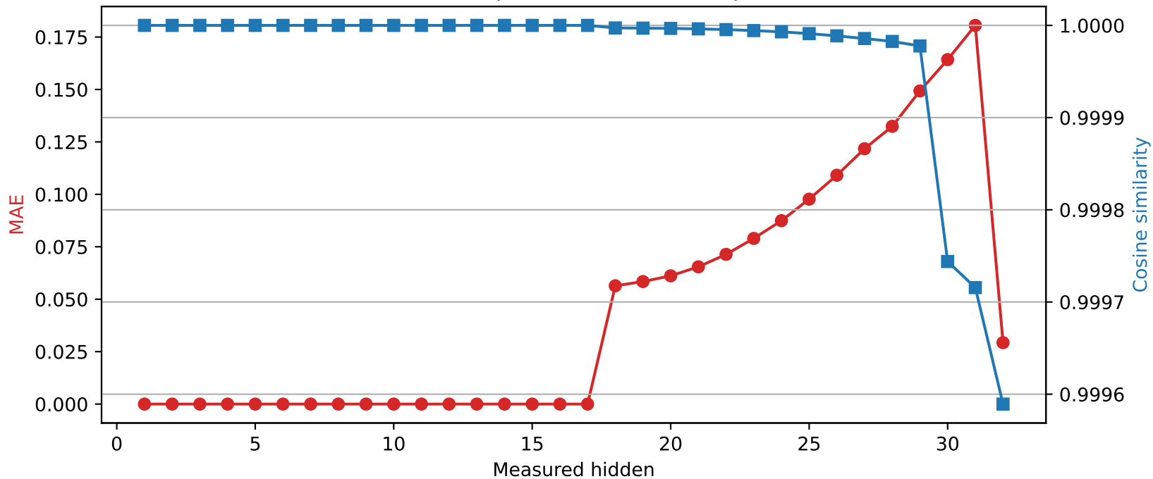
Phi-3-mini-4k-instruct | Quantized layer 17 | float16 \rightarrow int8
