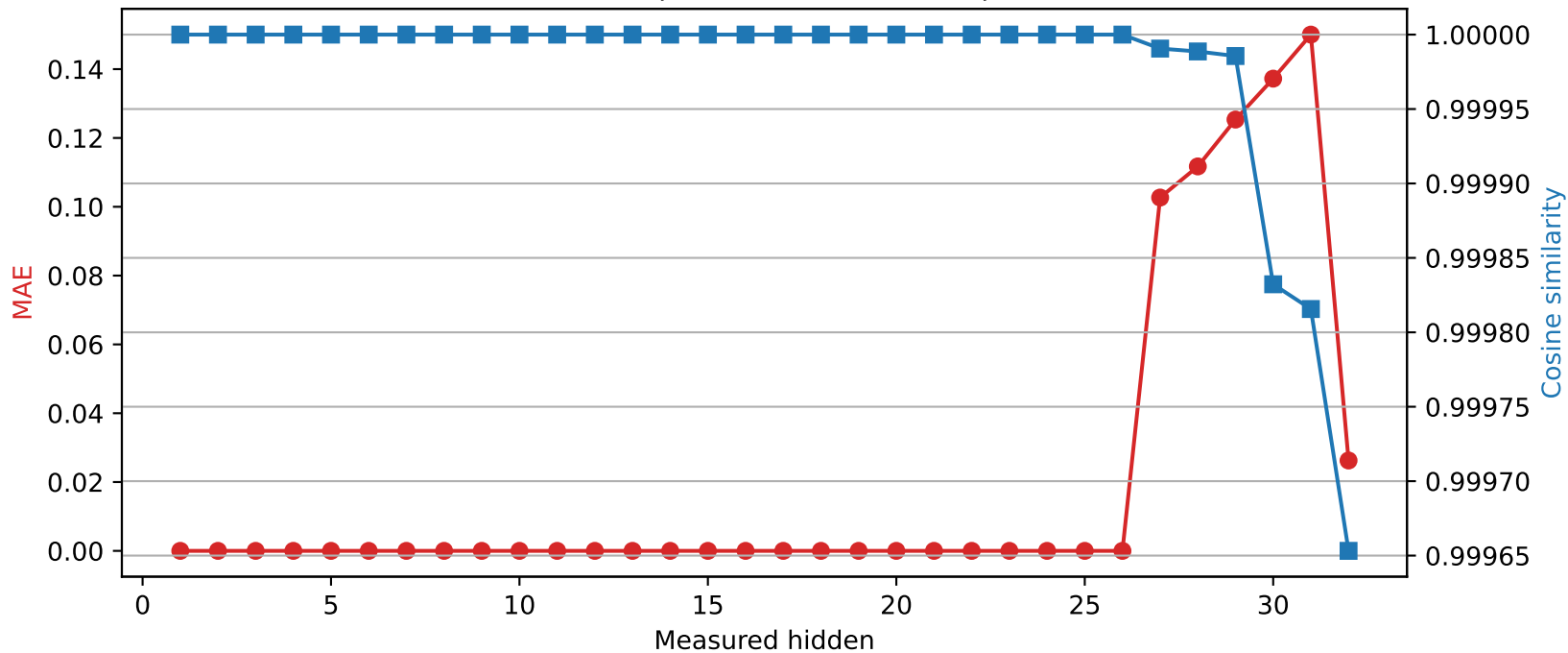
Phi-3-mini-4k-instruct | Quantized layer 26 | float16 → int8
