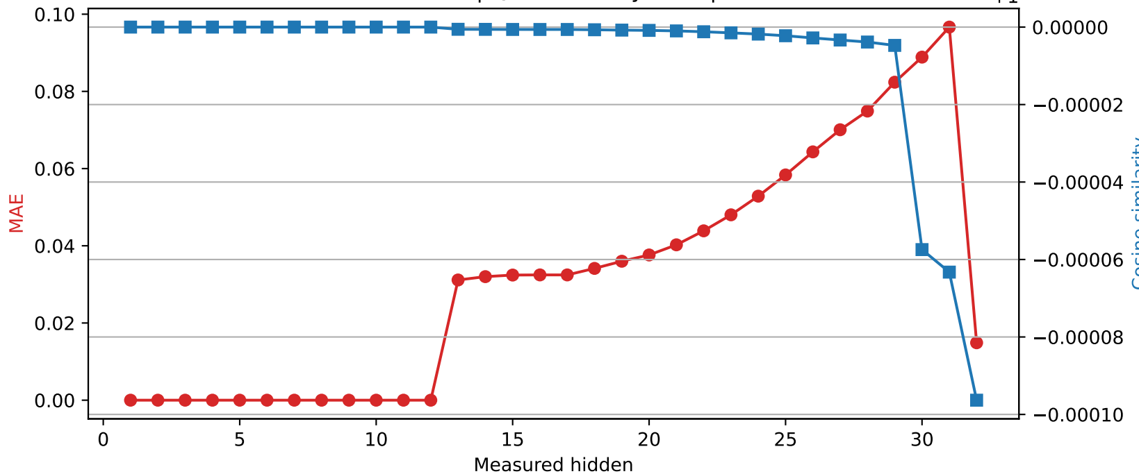
Phi-3-mini-4k-instruct | Quantized layer 12 | float16 → int8
