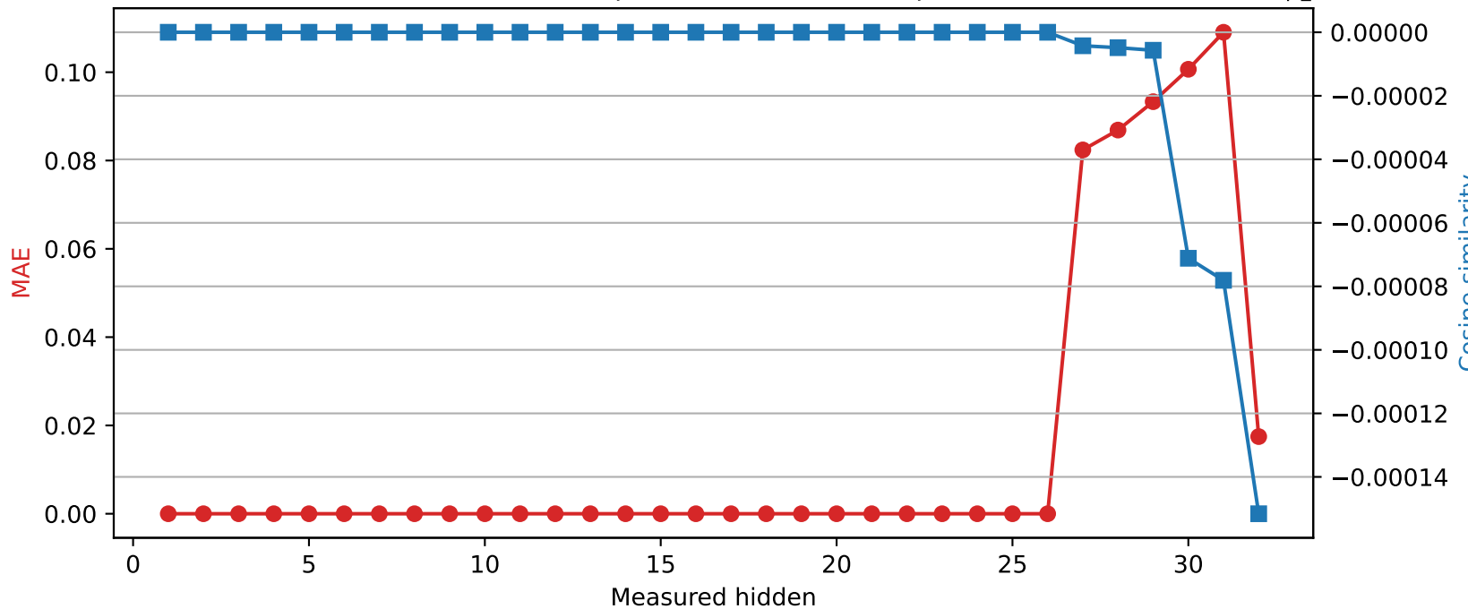
Phi-3-mini-4k-instruct | Quantized layer 26 | float16 \rightarrow int8
