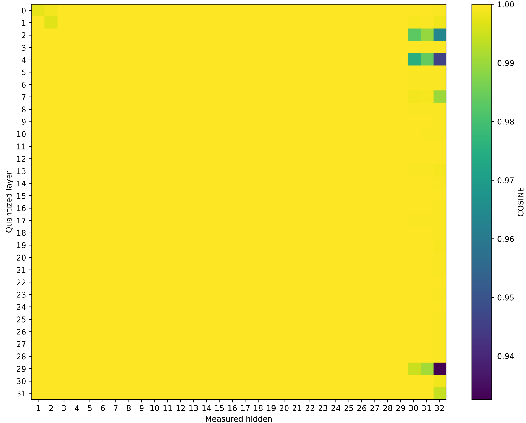
Model: Phi-3-mini-4k-instruct | float32 → int8
