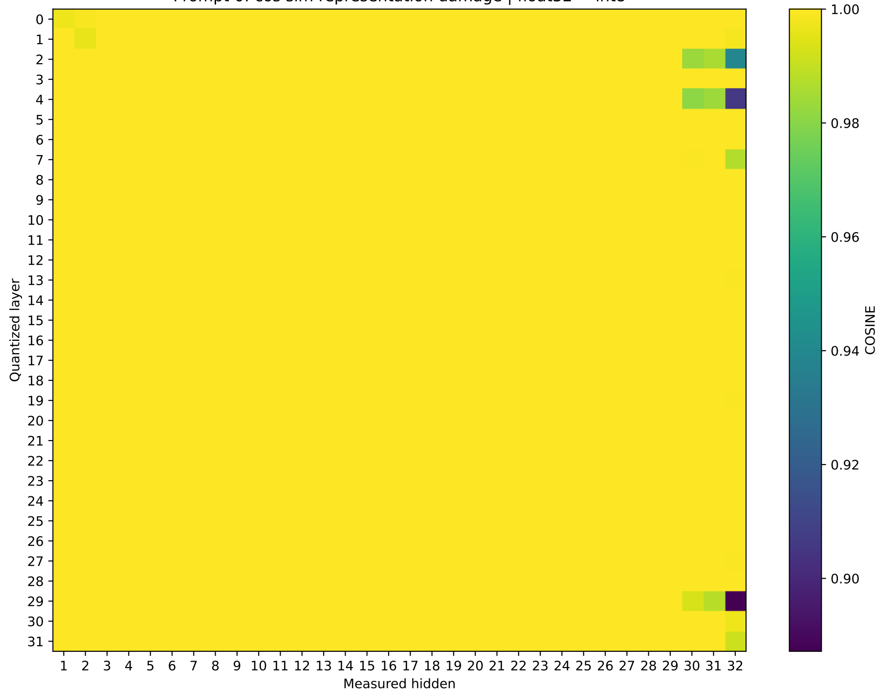
Phi-3-mini-4k-instruct Prompt 0: cos sim representation damage | float32 → int8
