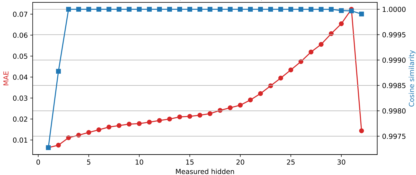
Phi-3-mini-4k-instruct | Quantized layer 0 | float32 \rightarrow int8
