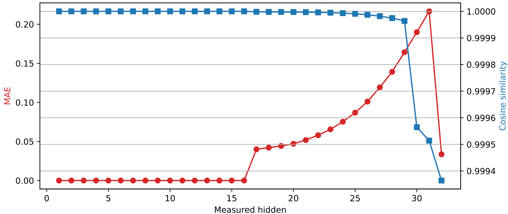
Phi-3-mini-4k-instruct | Quantized layer 16 | float32 → int8
