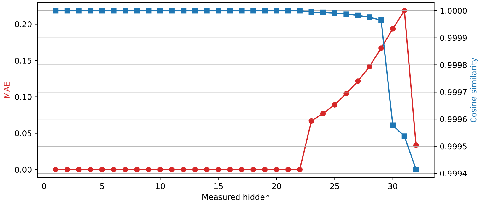
Phi-3-mini-4k-instruct | Quantized layer 22 | float32 → int8
