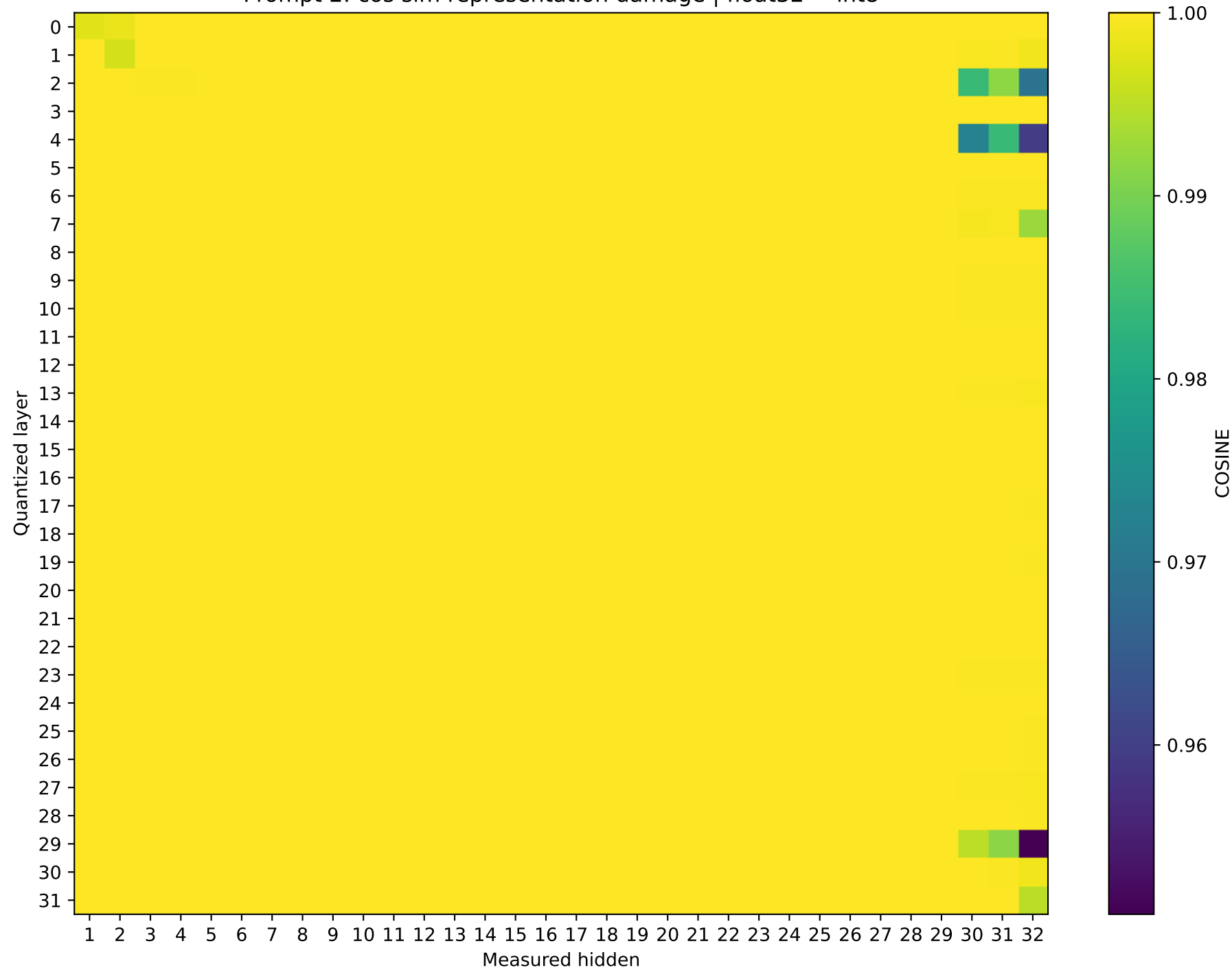
Phi-3-mini-4k-instruct Prompt 2: cos sim representation damage | float32 → int8
