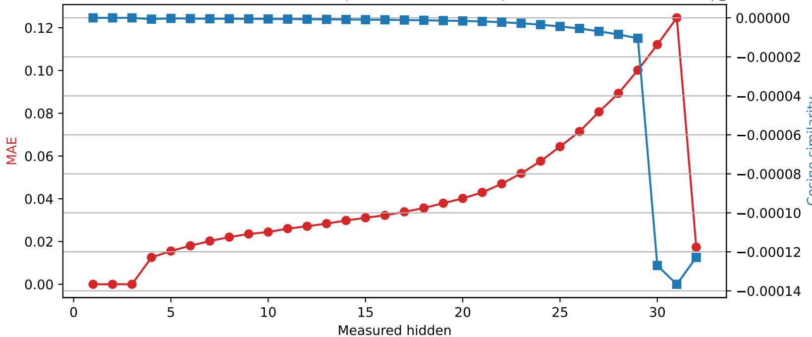
Phi-3-mini-4k-instruct | Quantized layer 3 | float32 \rightarrow int8
