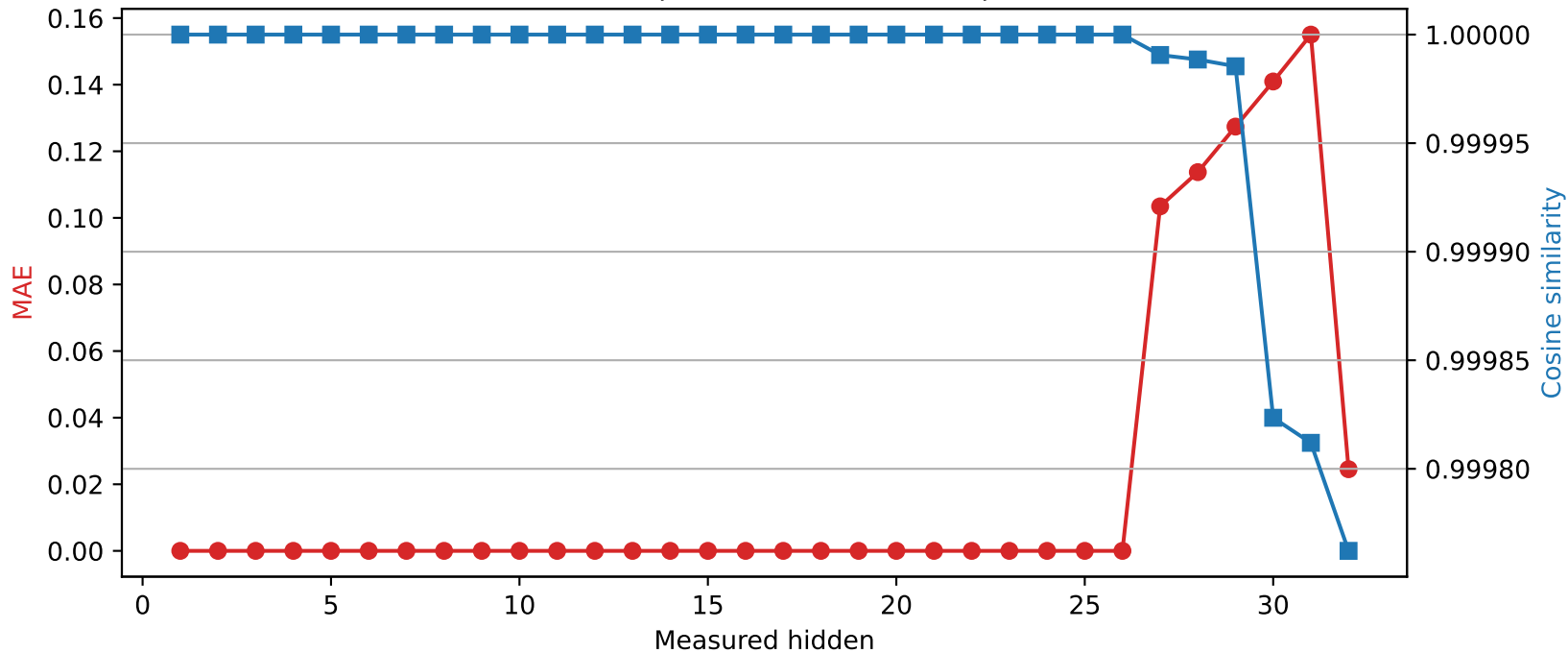
Phi-3-mini-4k-instruct | Quantized layer 26 | float32 \rightarrow int8
