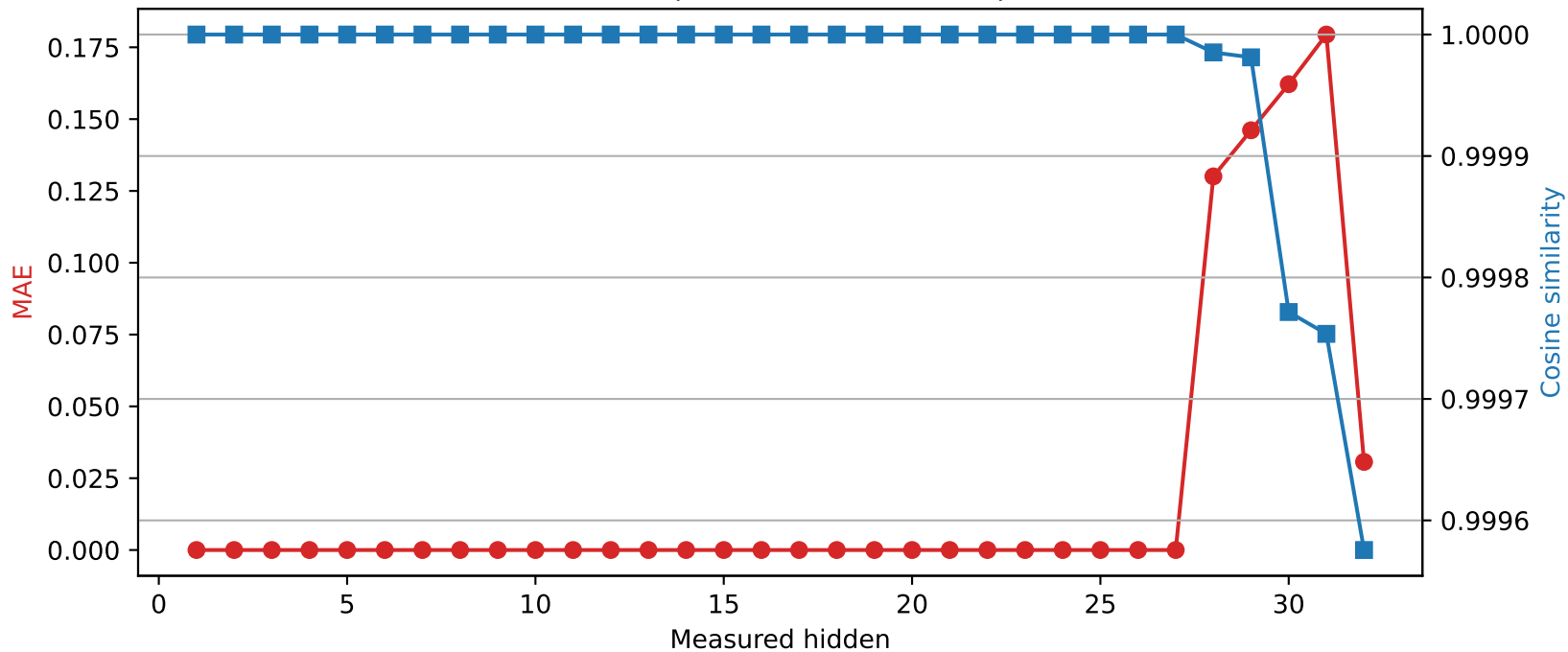
Phi-3-mini-4k-instruct | Quantized layer 27 | float32 → int8
