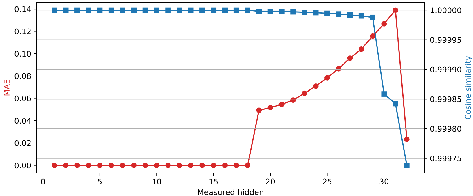
Phi-3-mini-4k-instruct | Quantized layer 18 | float32 \rightarrow int8
