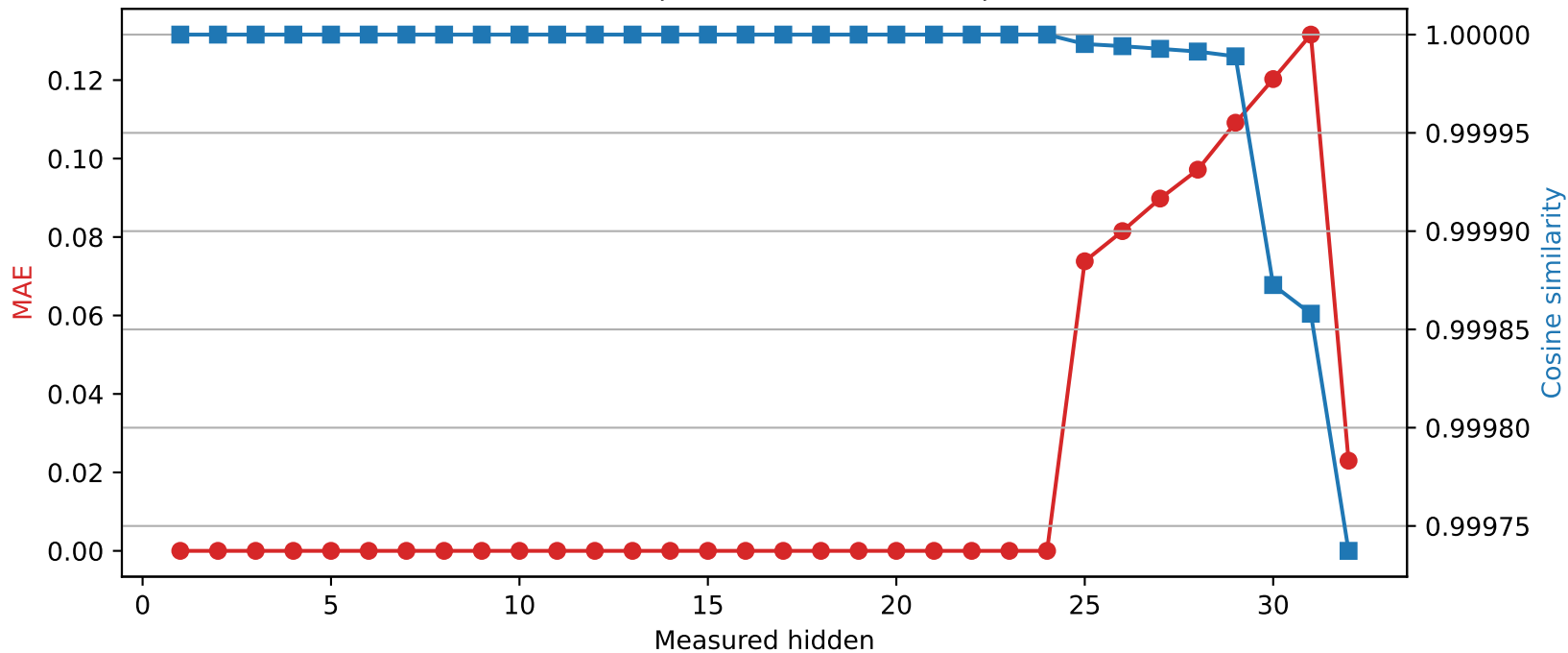
Phi-3-mini-4k-instruct | Quantized layer 24 | float32 → int8
