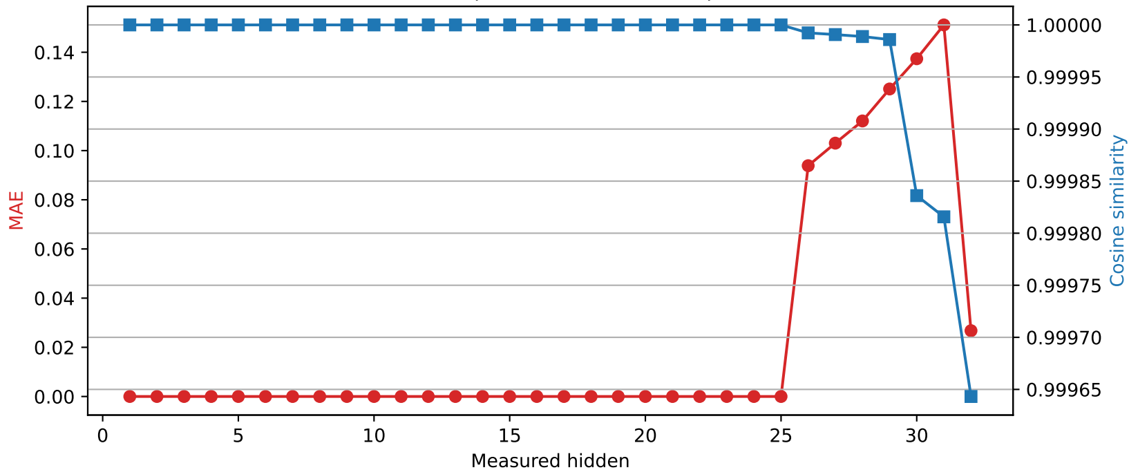
Phi-3-mini-4k-instruct | Quantized layer 25 | float32 → int8
