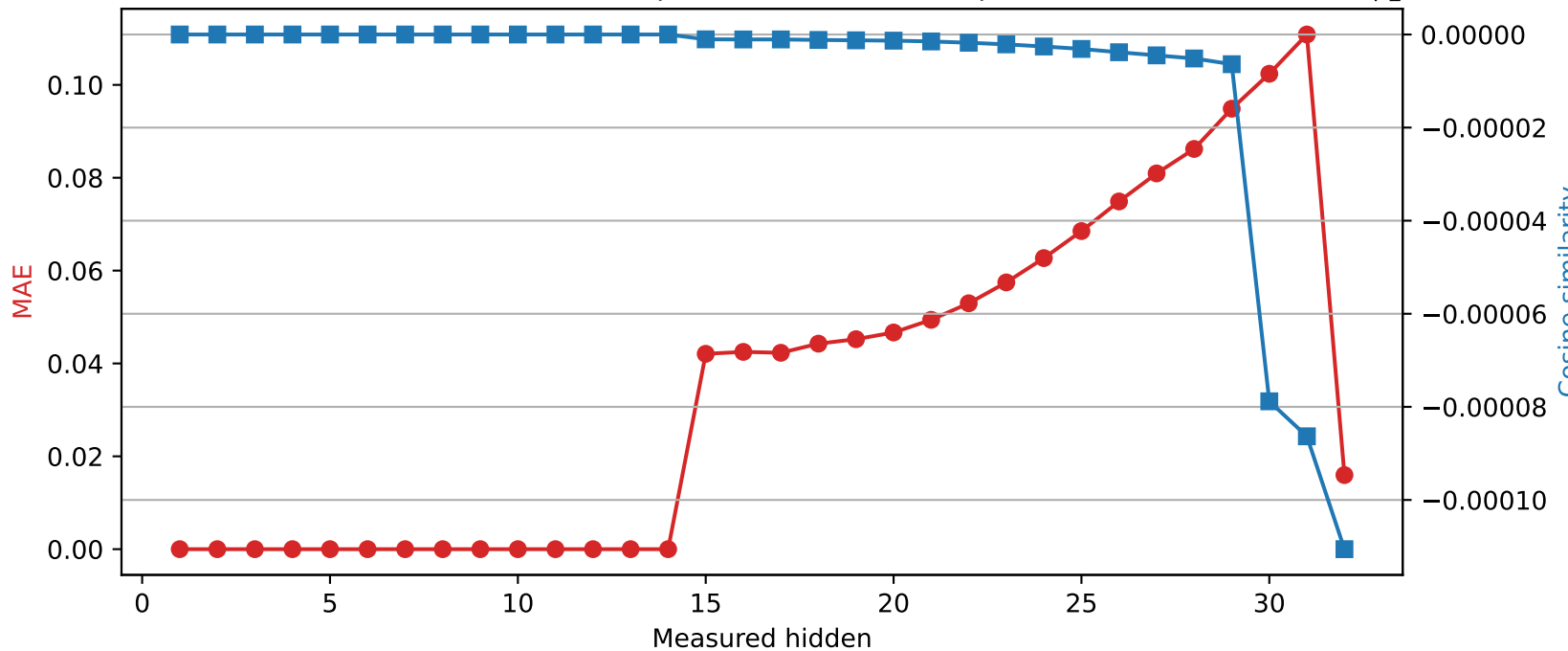
Phi-3-mini-4k-instruct | Quantized layer 14 | float32 → int8
