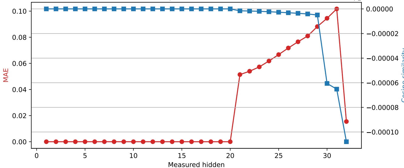
Phi-3-mini-4k-instruct | Quantized layer 20 | float32 \rightarrow int8
