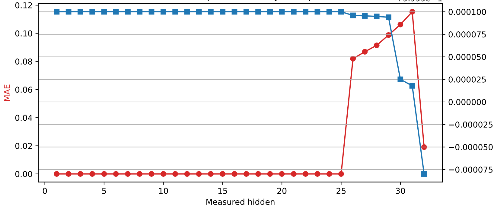
Phi-3-mini-4k-instruct | Quantized layer 25 | float32 \rightarrow int8
