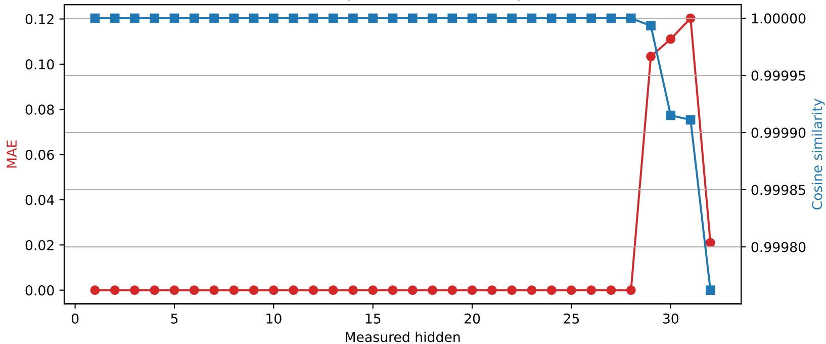
Phi-3-mini-4k-instruct | Quantized layer 28 | float32 → int8
