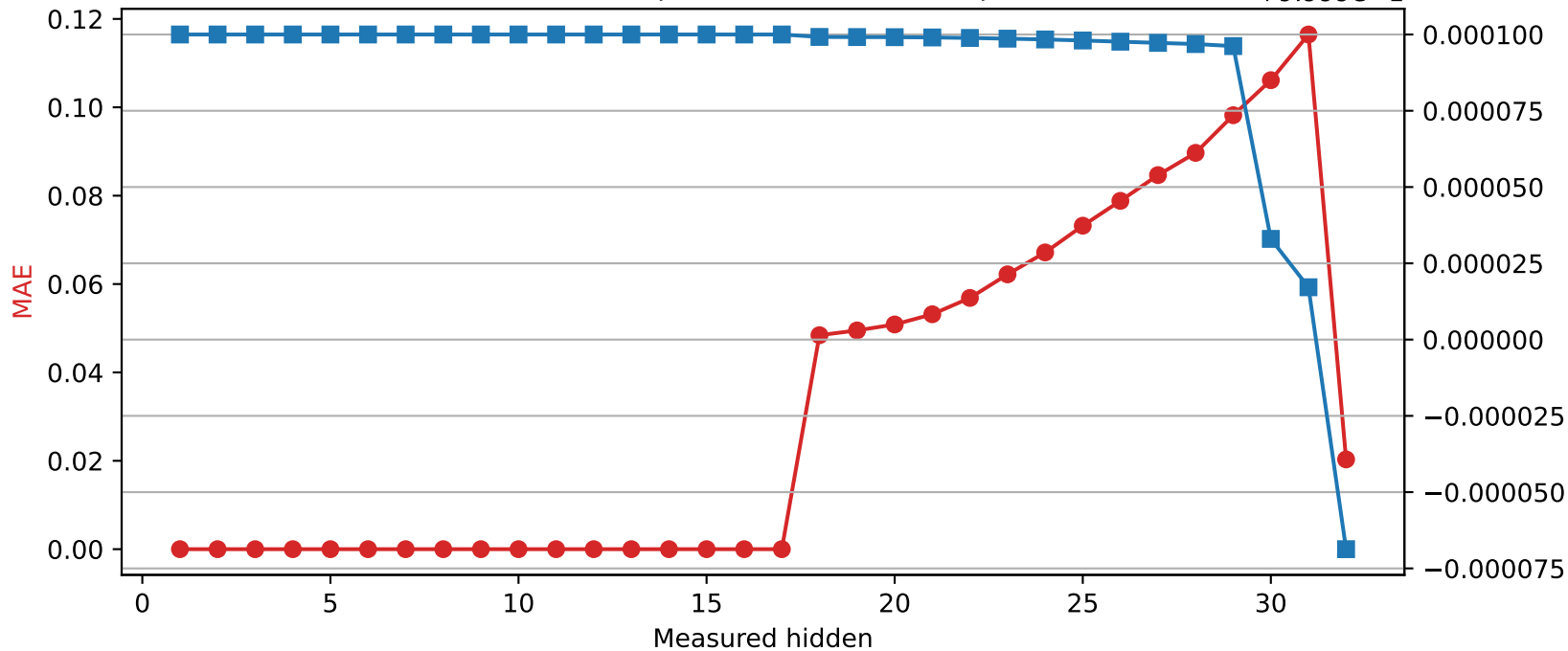
Phi-3-mini-4k-instruct | Quantized layer 17 | float64 → int8
