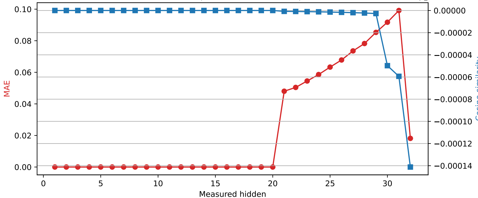
Phi-3-mini-4k-instruct | Quantized layer 20 | float64 → int8
