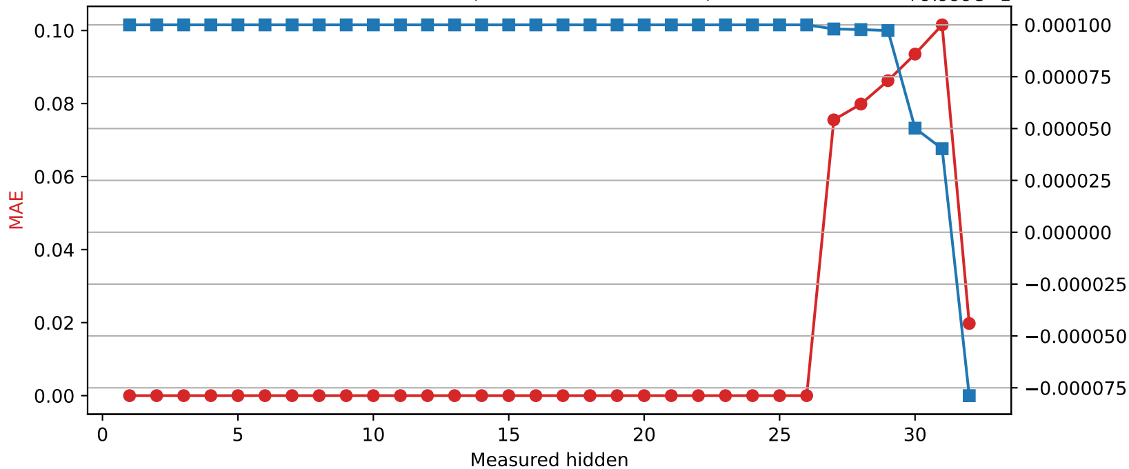
Phi-3-mini-4k-instruct | Quantized layer 26 | float64 \rightarrow int8
