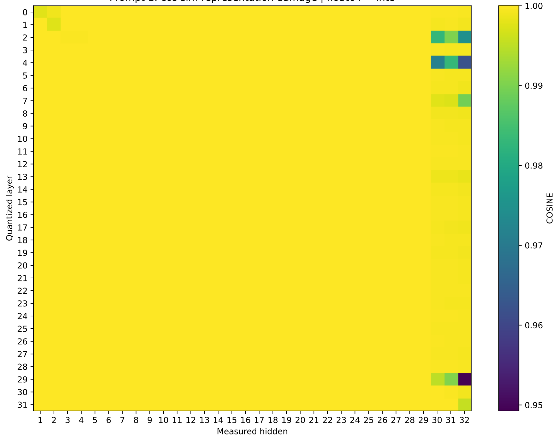
Phi-3-mini-4k-instruct Prompt 1: cos sim representation damage | float64 → int8
