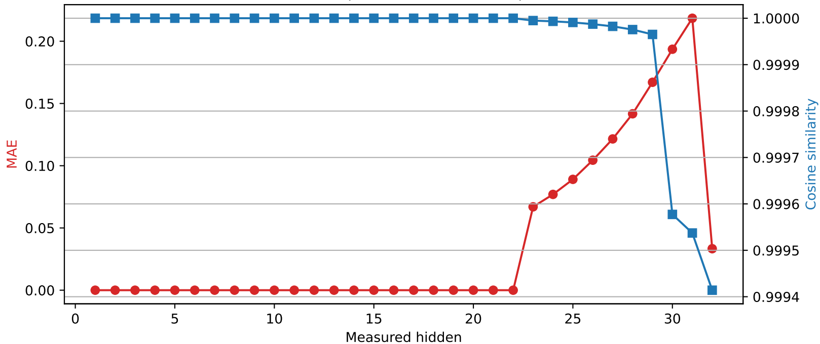
Phi-3-mini-4k-instruct | Quantized layer 22 | float64 → int8
