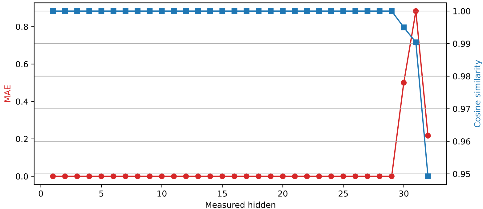
Phi-3-mini-4k-instruct | Quantized layer 29 | float64 → int8
