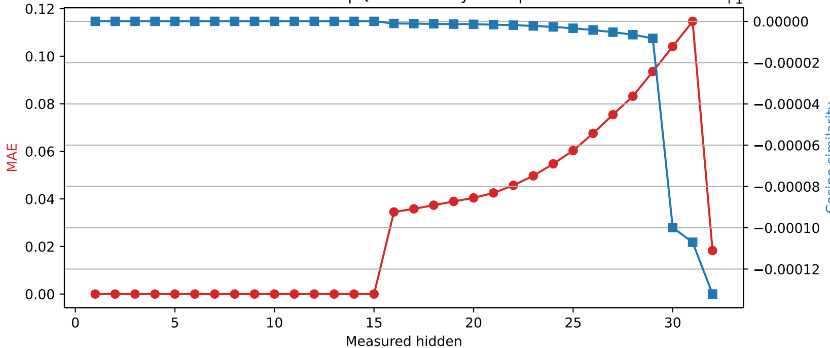
Phi-3-mini-4k-instruct | Quantized layer 15 | float64 → int8
