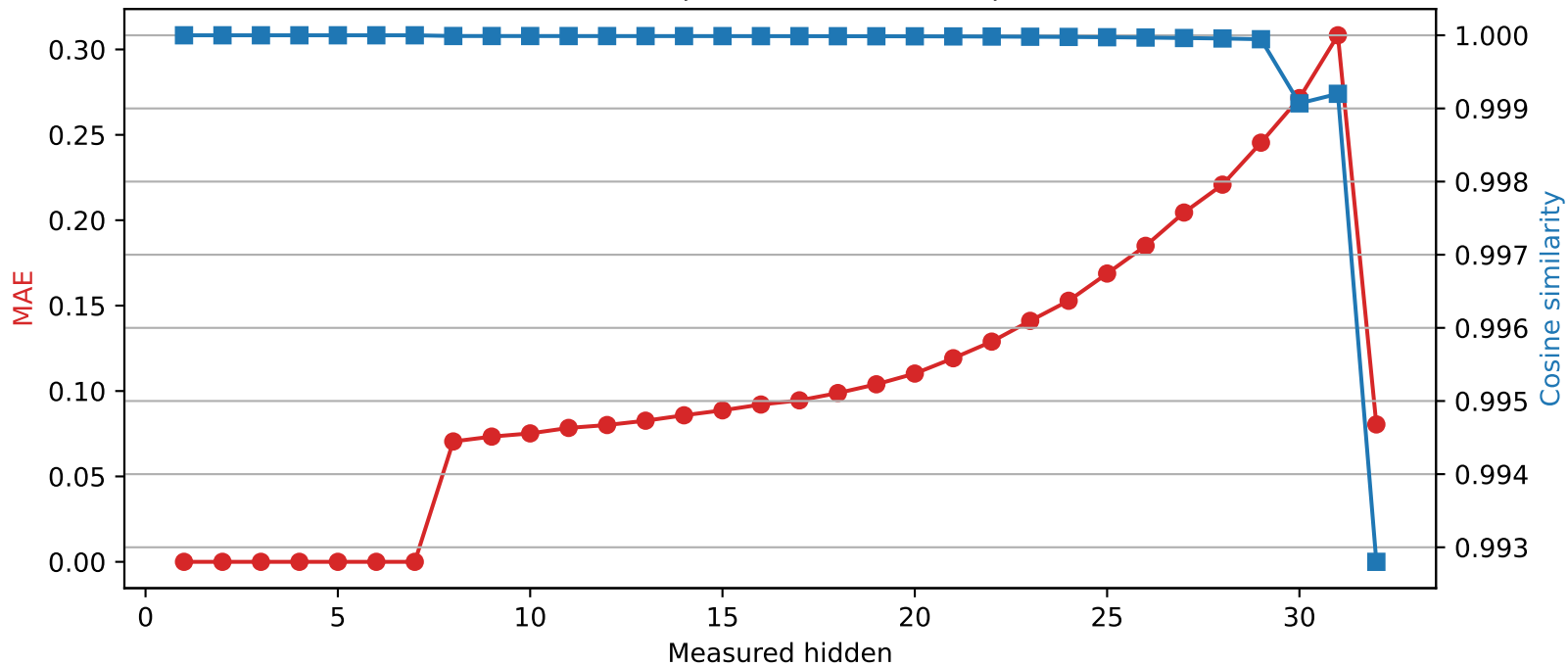
Phi-3-mini-4k-instruct | Quantized layer 7 | float64 → int8
