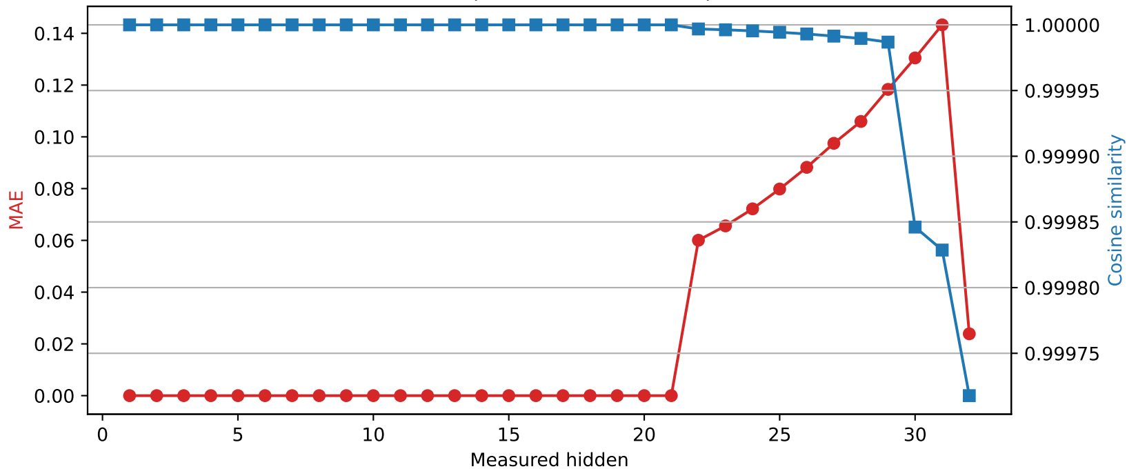
Phi-3-mini-4k-instruct | Quantized layer 21 | float64 → int8
