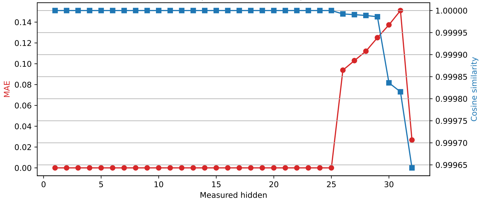
Phi-3-mini-4k-instruct | Quantized layer 25 | float64 → int8
