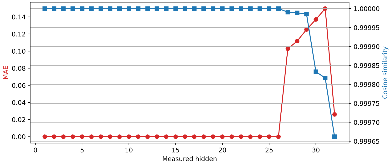
Phi-3-mini-4k-instruct | Quantized layer 26 | float64 → int8
