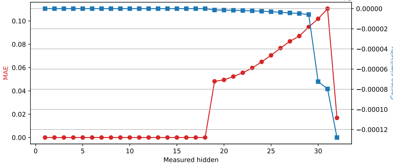
Phi-3-mini-4k-instruct | Quantized layer 18 | float64 → int8
