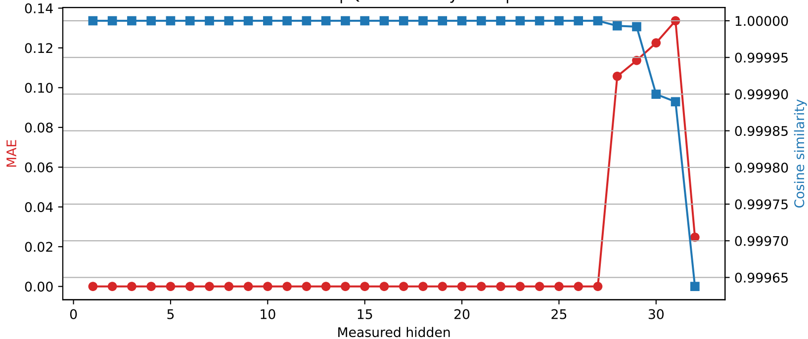
Phi-3-mini-4k-instruct | Quantized layer 27 | float64 → int8
