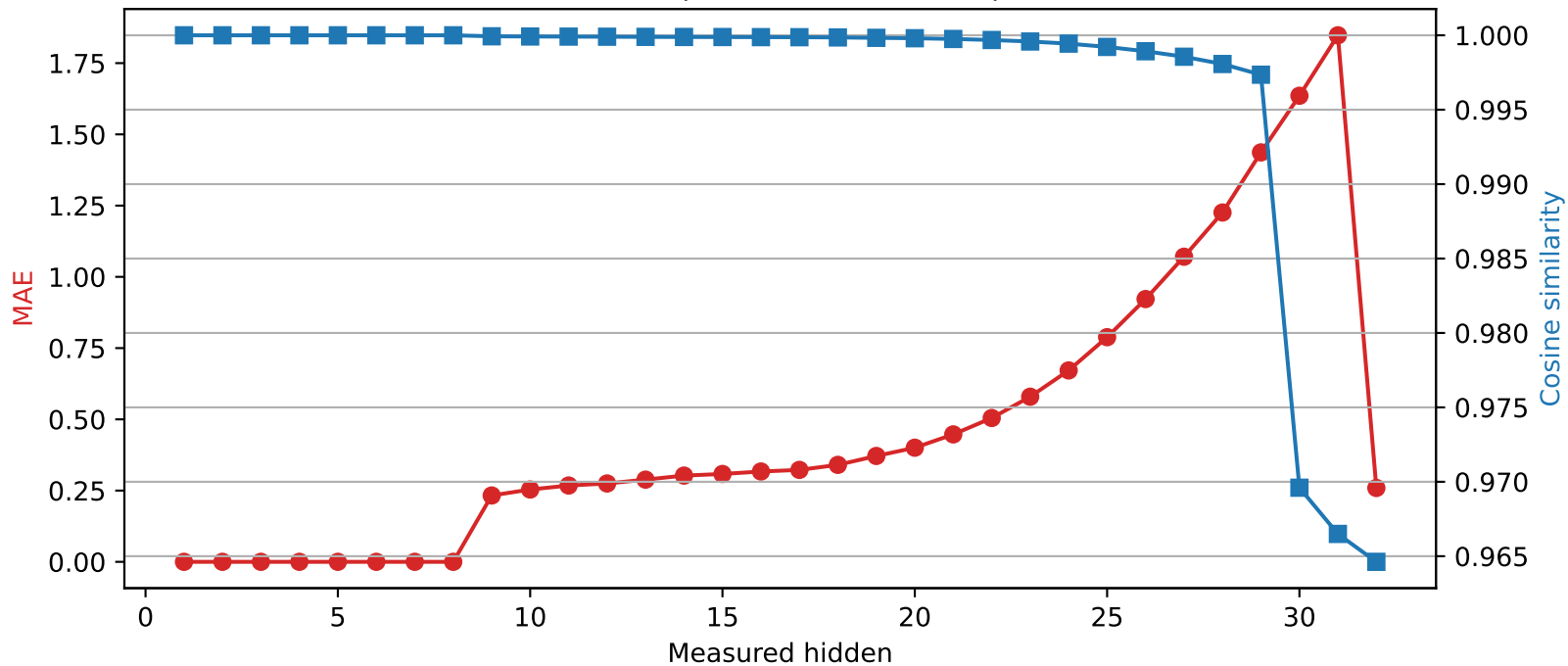
Phi-3-mini-4k-instruct | Quantized layer 8 | float16 \rightarrow int4
