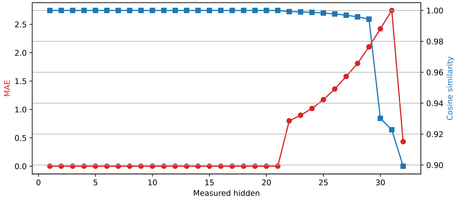
Phi-3-mini-4k-instruct | Quantized layer 21 | float16 \rightarrow int4
