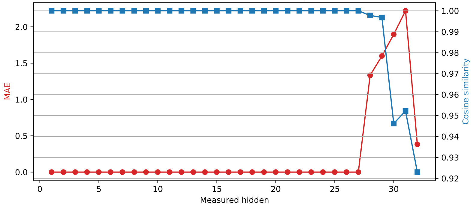
Phi-3-mini-4k-instruct | Quantized layer 27 | float16 \rightarrow int4
